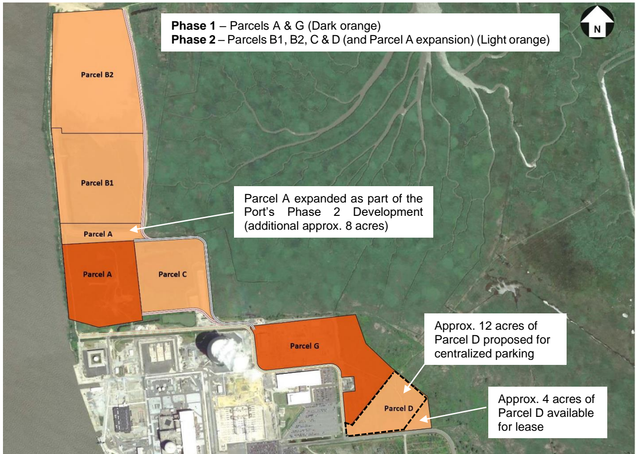
Figure 1 – The Port will be constructed in two phases
